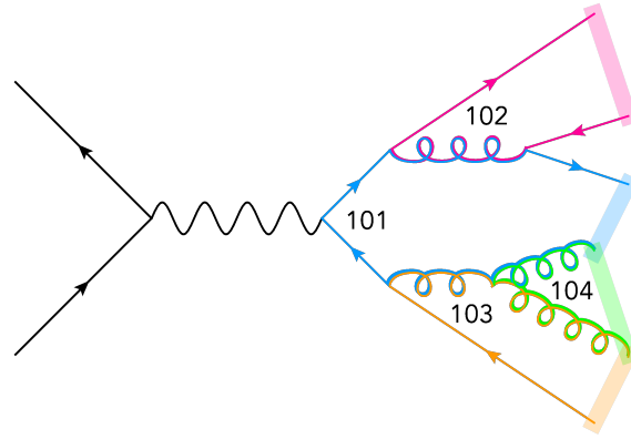
Figure 17: Illustration of LC colour flow in a simple e^+e^- \rightarrow q\bar{q} shower event. The shaded regions represent the resulting unique LC string topology.
